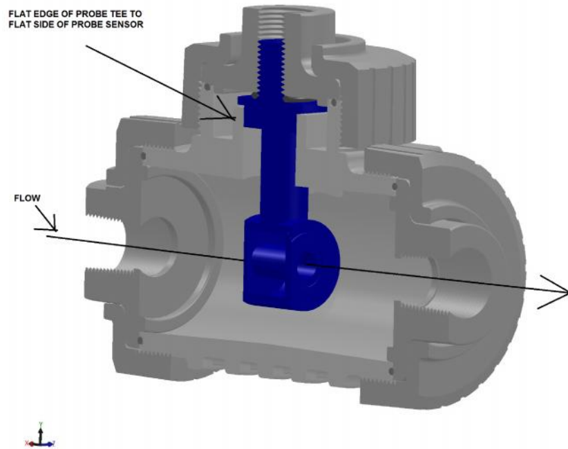
Fig. 1: Typical Installation
