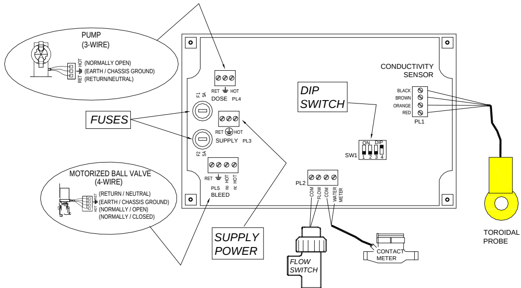
Fig. 3: Wire Connections 3
